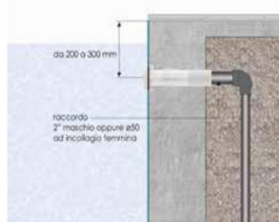
VAKUM TAČKASAPRODOROM VACUUM POINT WITH THROUGHWALL
