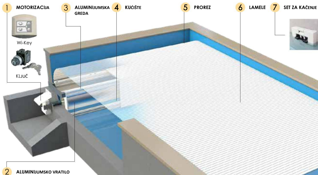
Rollinside verzija 2 strane, motor suvo kućište Rollinside 2 faces version, motor dry compartment
