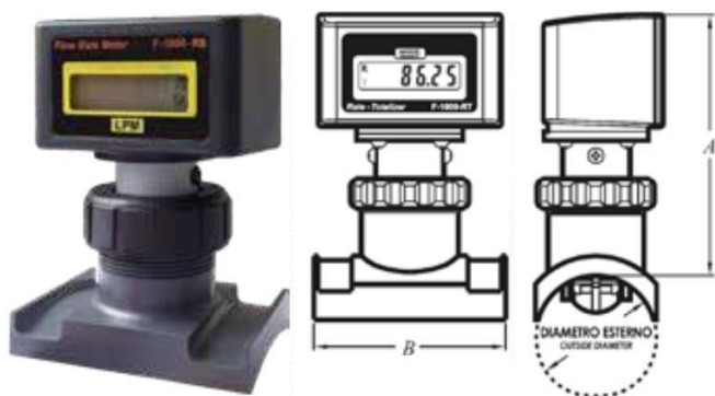
Instalacija / Installation INPUT 10 x I.D. - OUTPUT 5 X I.D.
