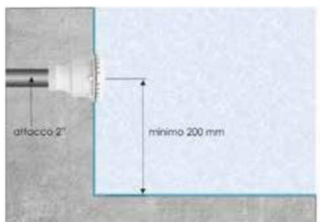
REGULATOR NIVOVA LEVEL CONTROLLER
